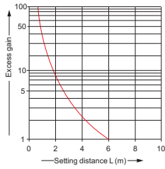
Correlation between setting distance and excess gain
