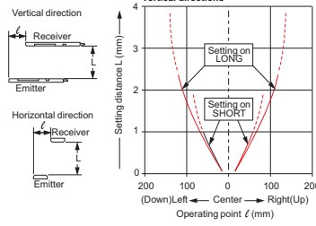
Parallel deviation
