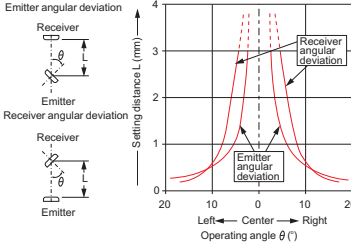
Angular deviation
