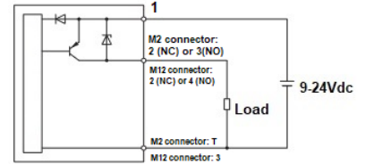
PNP wiring diagram
